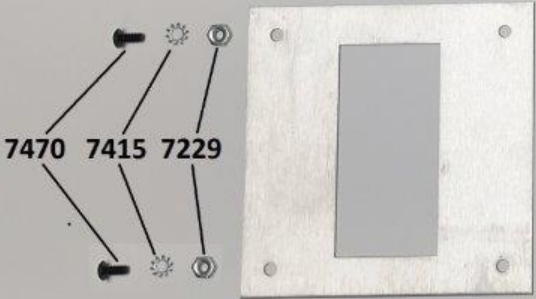
4133 Adapter Plate
